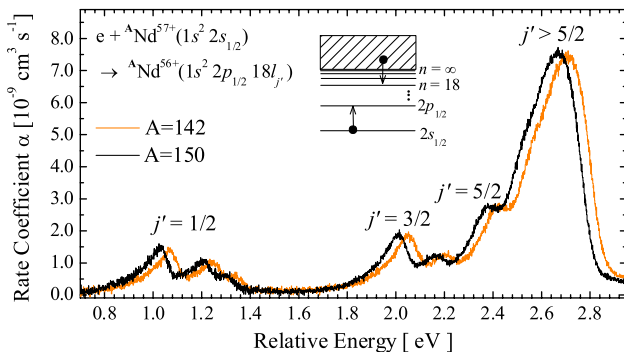
FIG. 1 (color online). Dielectronic recombination of the Li-like neodymium isotopes ^{142}\text{Nd}^{57+} (orange or gray line) and ^{150}\text{Nd}^{57+} (black line) in the energy range of the 1s^2 2p_{1/2} 18l_{j'} resonance groups. The labels indicate the individual fine structure components j' of the n = 18 Rydberg electron.
