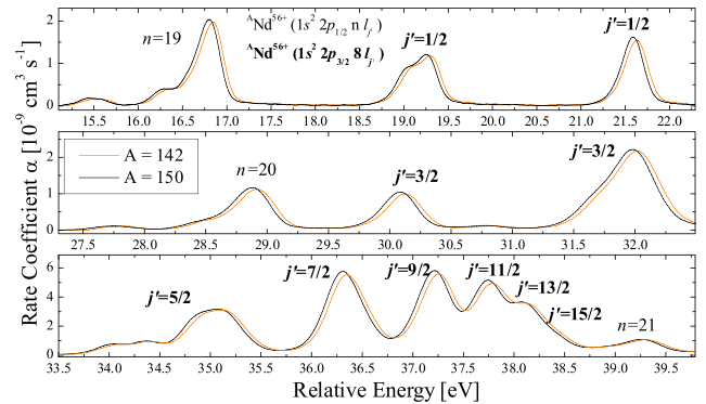
FIG. 2 (color online). Dielectronic recombination of A = 142 (orange or gray) and A = 150 (black) Li-like ^A\text{Nd}^{57+} . The labels n indicate the principal quantum number of the Rydberg electron of the 1s^2 2p_{1/2} nl_{j'} configurations and the bold labels j' denote the fine structure components of the 1s^2 2p_{3/2} 8l_{j'} resonances.
