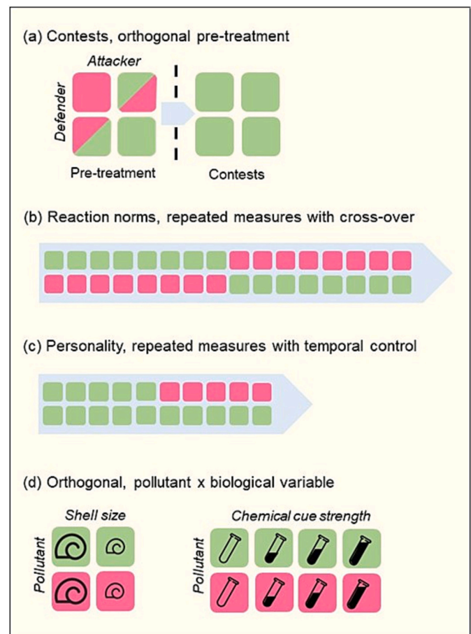
Fig. 3. Some core experimental designs used to test for the effects of pollutants on the behaviour of hermit crabs. Green boxes represent control treatments where pollutants are absent and magenta boxes indicate treatments where crabs are exposed to pollutants. Where relevant, blue shading represents the chronology of the experiment. Where this is absent, data were collected simultaneously across treatment groups. Note that some details (e.g. number of repeated measures) vary across studies.
