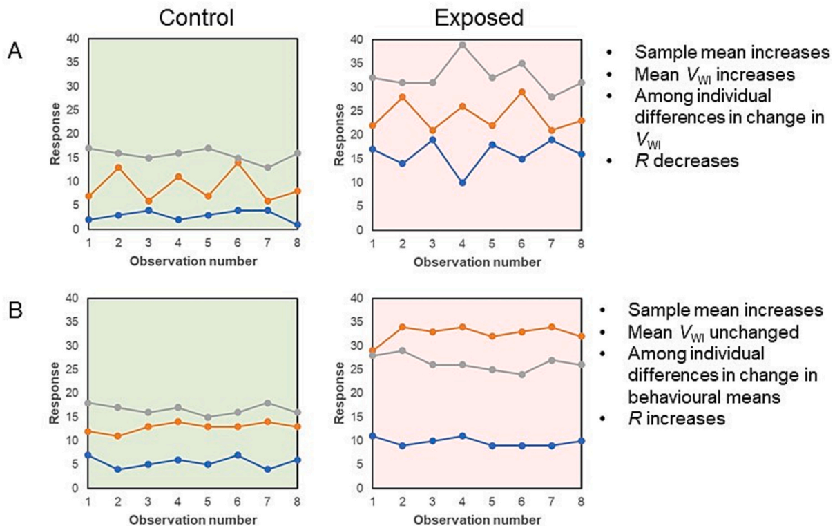
Fig. 2. Overview of levels of analysis for the effects of pollution on behaviour studied within the animal personality framework, illustrated with hypothetical data from two experiments A and B. Dots joined by lines show datapoints collected repeatedly from three individuals denoted by different colours. Green plots denote control treatments and pink plots denote exposure to a pollutant. In both cases, each individual is exposed to both conditions – see Fig. 3 (b and c) for examples of experimental designs needed to control for chronological effects in such experiments. In scenario A, during the control treatment the orange individual shows greater V_{WI} compared to the grey and blue individuals. When exposed to a pollutant the sample mean behavioural response is greater compared with the control. Additionally, the sample mean of V_{WI} has increased but this increase has been more marked in the grey and blue individuals compared with the orange individual. As a consequence of net elevation in V_{WI} , repeatability ( R ), is reduced under exposure to the pollutant. In scenario B, R is greater under control conditions compared with the data collected under control conditions during experiment A. This is due to the lower V_{WI} under control conditions in experiment B. V_{WI} does not change under exposure to the pollutant but the sample mean response has again increased. However, there is significant variation among individuals in how the pollutant affects their behaviour, such that they show different behavioural reaction norms (BRN). The orange individual has increased its response by a large amount, the grey individual by a moderate amount and the responses of the blue individual are largely unchanged. Additionally, while V_{WI} is unchanged, V_{BI} has increased, leading to an increase in R .
