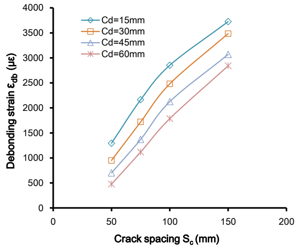
Fig. 8. Effect of crack spacing on debonding strain
