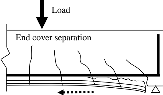
Fig. 1 Schematic of end cover separation
