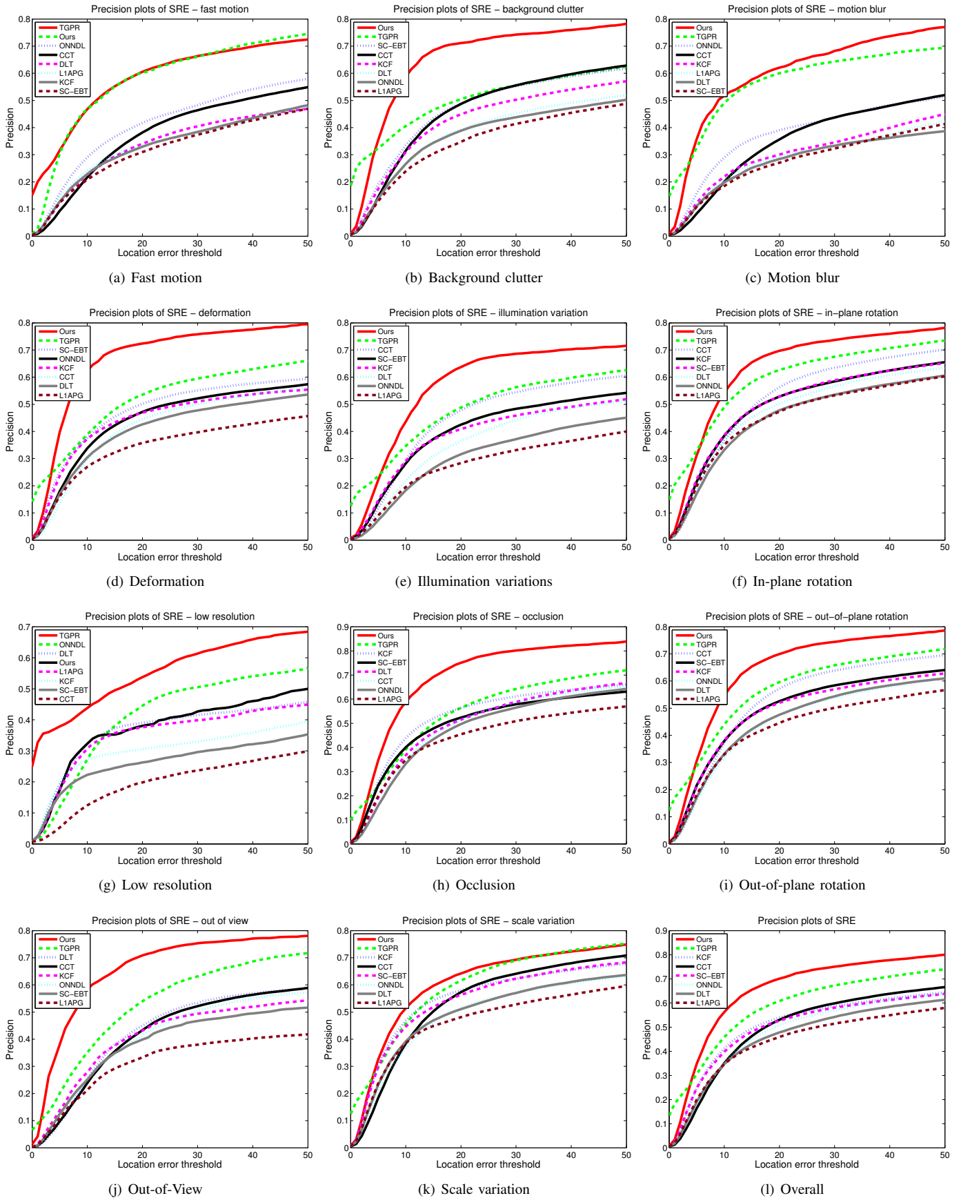
Fig. 4. Precision plots for the challenges considered in this work.
