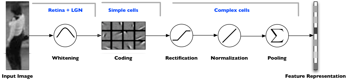
Fig. 1. The architecture of the proposed biologically inspired appearance modeling framework (LGN = Lateral Geniculate Nucleus).
