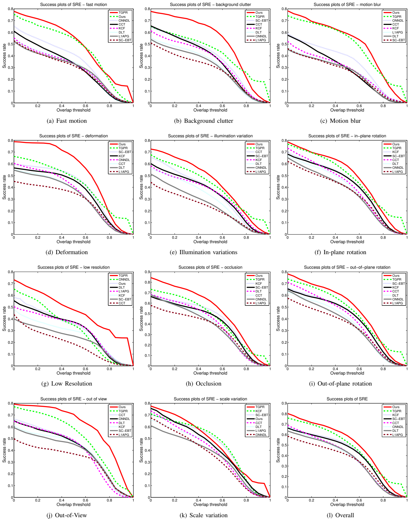
Fig. 3. Success plots for the challenges considered in this work.
