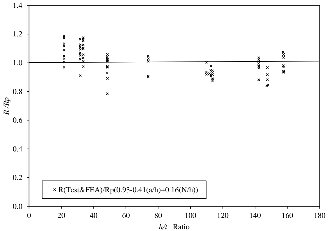
Fig.8 Comparison of strength reduction factor for centred hole where flanges fastened to bearing plates
