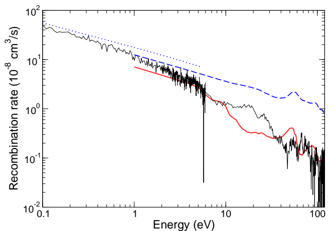
FIG. 2. (Color online) The graph shows the total rate of electron resonant capture by W^{20+} , calculated using statistical theory (dotted blue line, Ref. [15]; dashed blue line, Ref. [16]), and the calculated recombination rate (thick solid red line), obtained by including the effect of the nonunit fluorescence yield [16]. Thin solid black line is the experimental recombination rate from Ref. [20].
