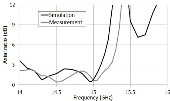
Fig. 13. Axial ratio (simulated and measured) of finite antenna with a patch antenna source.
