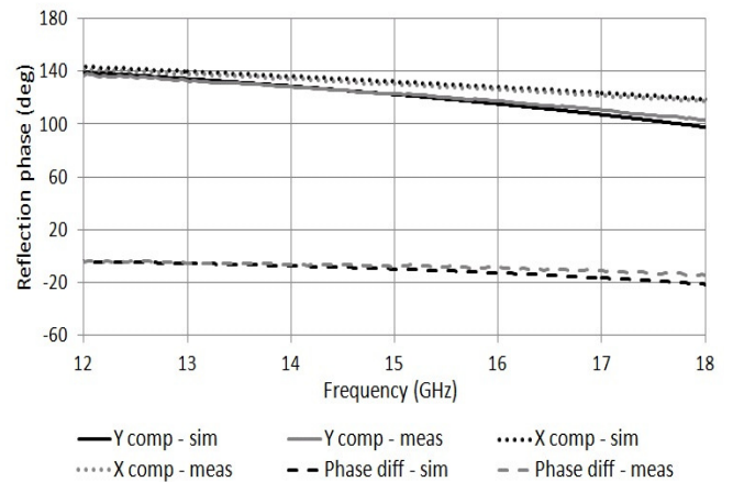
Fig. 10. Simulated and measured reflection phase (y- and x-components plus phase difference) of HIS with L_{y\text{his}} = 2.3
