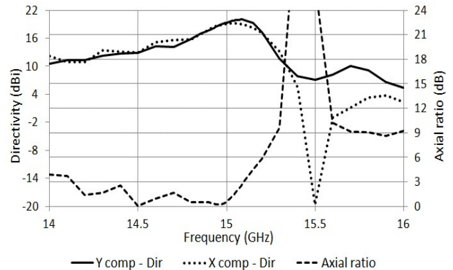
Fig. 7. Simulated directivity (y- and x-components) and axial ratio of finite antenna with simple dipole model source.
