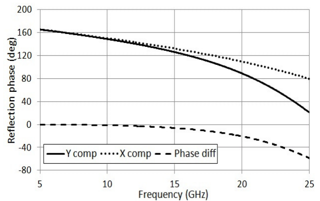
Fig. 5. Simulated reflection coefficient phase of high impedance surface ground plane – y- and x-components plus phase difference.
