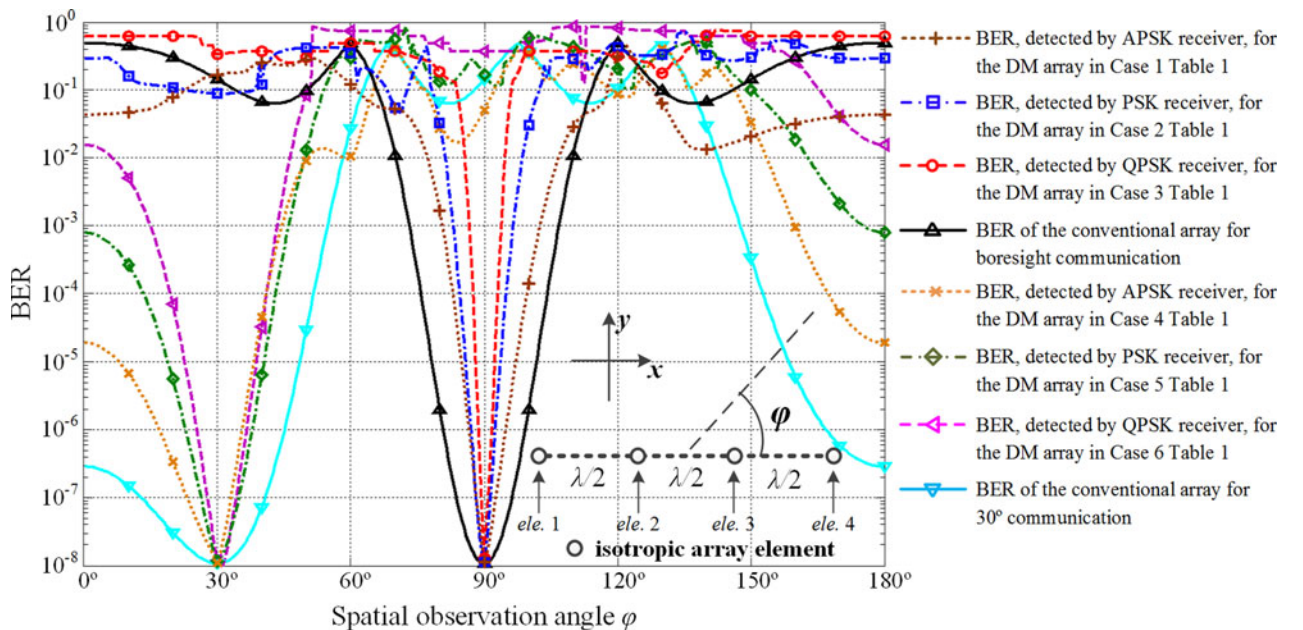
Fig. 4. BER performance, detected by the corresponding type receivers, of the synthesized 1 \times 4 DM transmitter arrays as well as the 1 \times 4 conventional arrays optimized for broadside and 30^\circ secure communications with the system settings in Table 1.
