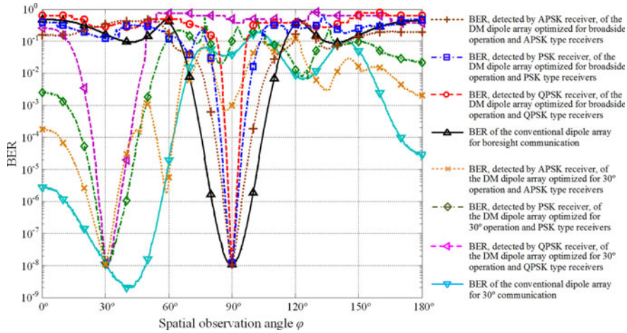
Fig. 11. BER performance, detected by the corresponding type receivers, of the 1 × 4 DM dipole transmitter arrays as well as the 1 × 4 conventional dipole arrays for broadside (90°) and 30° secure communications.
