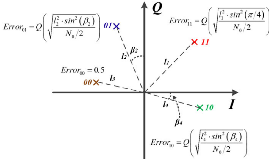
Fig. 3. Illustration of Error_{xy} and \beta_i for the QPSK receiver case.
