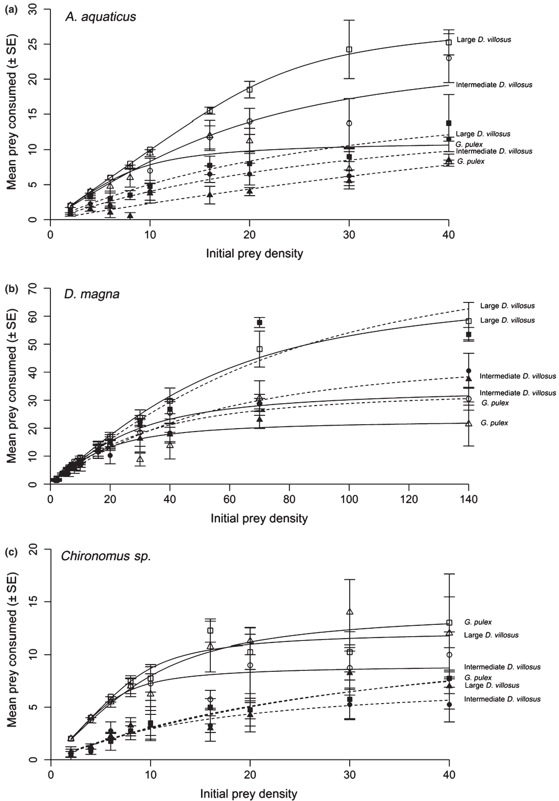
Fig. 3 Functional responses of large Dikero gammarus villosus (squares), intermediate D. villosus (circles) and Gammarus pulex (triangles) in simple (open symbols, solid line) and complex (closed symbols, dashed line) substrate arenas with (a) Asellus aquaticus , (b) Daphnia magna and (c) Chironomus sp. prey.
