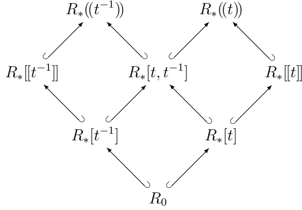
FIGURE 1. The collection of rings and their inclusion relation
