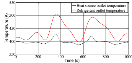
Fig.2. Outlet temperatures of dynamic evaporator model.
