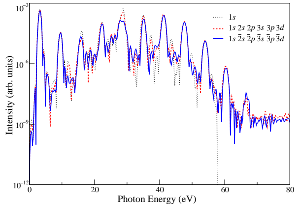
FIG. 2: (Color online) The length form harmonic spectrum of He in a 390 nm, 4 \times 10^{14} Wcm ^{-2} , 3-2-3 laser field, using as a residual ion description, the 1T (black, dotted line), 6T (red, dashed line), and 6P (blue, solid line) models (See Fig. 1 for details). Results from the 1T model provide a reasonable approximation to results from the more detailed descriptions especially in the cutoff region. There is also good agreement for the first harmonic when compared with the large discrepancy in Fig. 1.
