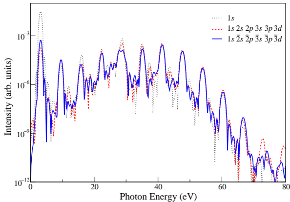
FIG. 1: (Color online) The harmonic spectrum (up to a constant of proportionality) as calculated from the dipole acceleration for He in a 390 nm, 4 \times 10^{14} Wcm ^{-2} , 3-2-3 laser field, using as a model residual ion description, the 1s state (black, dotted line), the 1s, 2s, 2p, 3s, 3p, 3d states (red, dashed line), and the 1s, \bar{2}s , \bar{2}p , \bar{3}s , \bar{3}p , \bar{3}d pseudostates (blue, solid line). The single state model provides a reasonable approximation to the more detailed descriptions beyond the first harmonic where there is a large discrepancy between the spectra.
