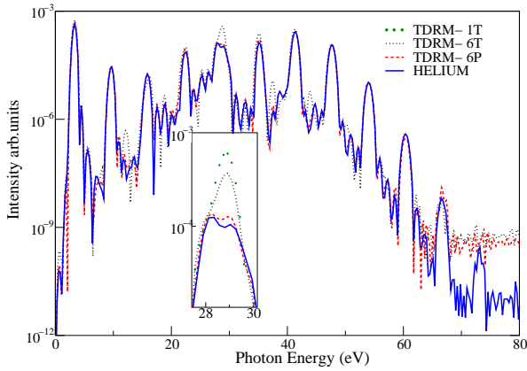
FIG. 5: (Color online) The harmonic spectra as calculated from the dipole length produced from the 6T (black, dotted line) and 6P (red, dashed line) He models for TDRM, and from the HELIUM code (blue, solid line). The 6P and 6T spectra agree with the HELIUM spectrum to within 20% and 30% respectively up to the 21st harmonic peak (except at the 9th and 11th harmonics for the 6T spectrum). Inset: Both the 6P and HELIUM models have a structured peak at the 9th harmonic. The 1T (green circles) and 6T spectra do not.
