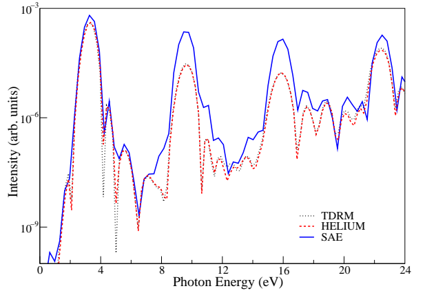
FIG. 6: (Color online) The low energy region of the dipole velocity harmonic spectrum produced from the 6P He model in TDRM (black, dotted line), and the length form harmonic spectra from the HELIUM code (red, dashed line), and its SAE derivative (blue, solid line). The TDRM and HELIUM spectra are indistinguishable, but the SAE spectrum overestimates the harmonic spectrum at low energies.
