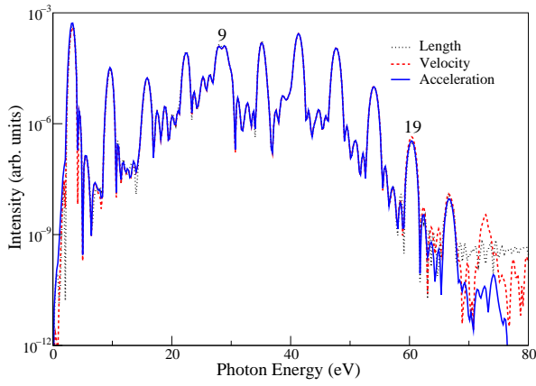
FIG. 3: (Color online) The harmonic spectrum of a pseudostate (6P) He target in a 390 nm, 4 \times 10^{14} Wcm ^{-2} 3-2-3 laser field, as calculated from the dipole length (black, dotted line), velocity (red, dashed line) and acceleration (blue, solid line). Agreement to within 20% is found between all three spectra up to the 19th harmonic peak (60 eV). The spectra diverge beyond this.
