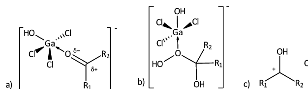
Scheme 2 Electrophilic activation of (a) ketone by Lewis acid, (b) the intermediate by Lewis acid, and (c) ketone by Brønsted acid in Baeyer-Villiger oxidation with hydrogen peroxide. Adapted from ref. 2.
