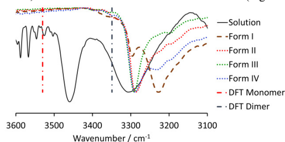
Figure 2 N-H region of the normalised transmission FTIR spectra of a 0.542 M solution of OCB in chloroform and the four crystal forms.
