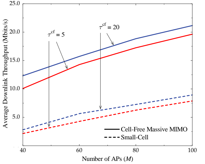
Fig. 11. The average downlink net throughput versus the number of APs for different \tau^{cf} . Here, K = 20 .
