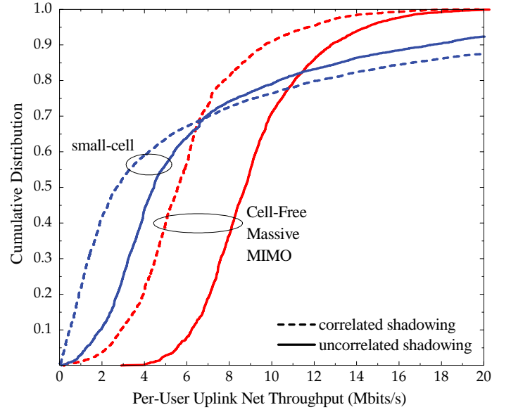
Fig. 8. The same as Figure 7 but for the uplink, and \tau^{\text{cf}} = \tau_u^{\text{sc}} = 20 .
