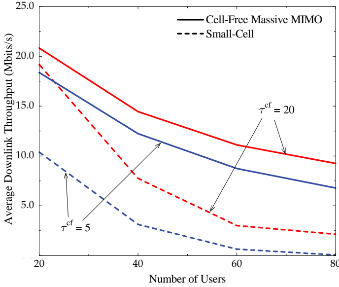
Fig. 10. The average downlink net throughput versus the number of users for different \tau^{cf} . Here, M = 100 .
