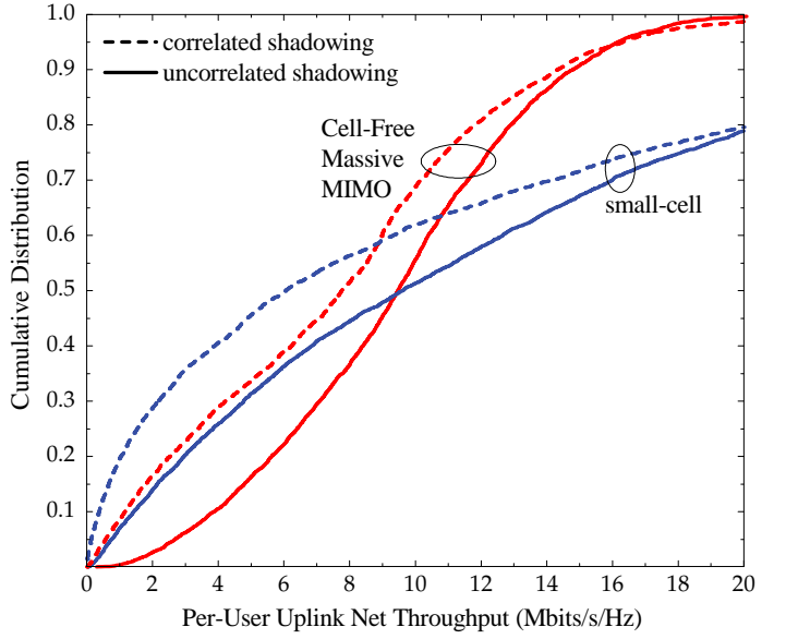
Fig. 6. The same as Figure 5 but for the uplink, and \tau_u^{cf} = \tau_u^{sc} = 20 .
