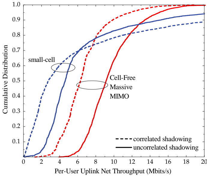
Fig. 4. The same as Figure 3 but for the uplink, and \tau_u^{cf} = \tau_u^{sc} = 20 .
