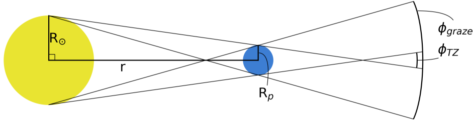
Figure 1. The transit zone of a planet (centre) projected out from the Sun (left). Sizes and distance not to scale.
