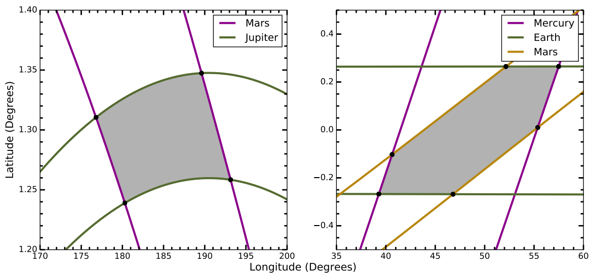
Figure 3. Examples of regions where the non-grazing transit zones intersect, given in ecliptic coordinates. The black circles are the points where the lines intersect – equatorial coordinates of these points are given in Appendix A for all overlap regions.
