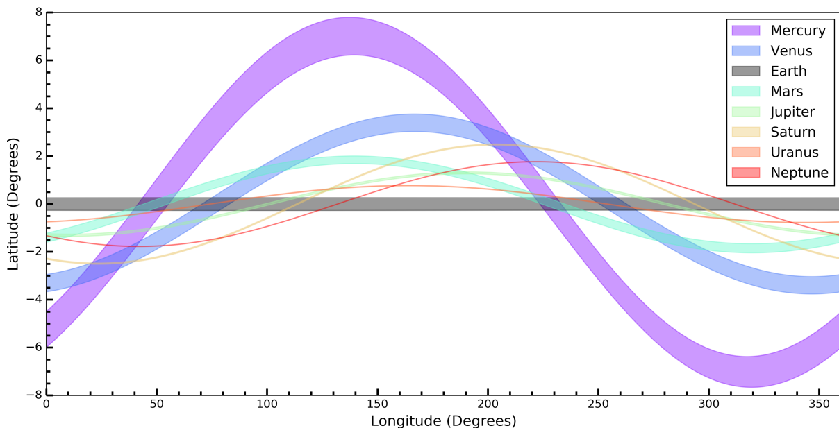
Figure 2. Projections of the transit visibility zones (non-grazing) of all the Solar System planets in heliocentric ecliptic coordinates. Each planet’s transit zone is defined as a coloured bounded region.
