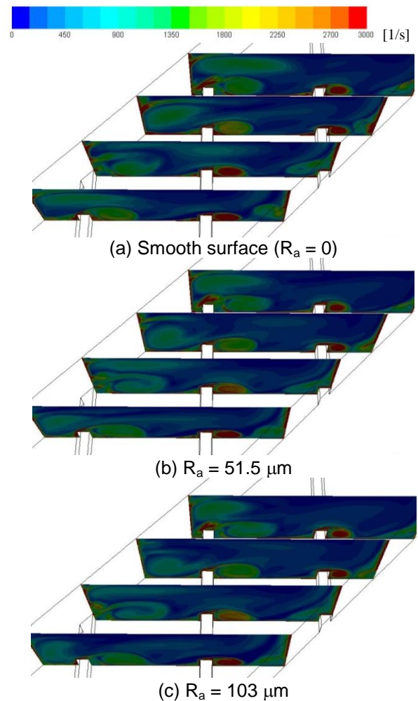
Figure 4 – Vorticity contours to compare the vortical flows in the ribbed duct
