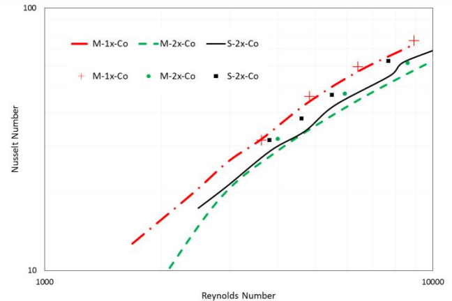
Figure 2 – Comparison of experimental and simulated results (Line represents experimental data and point represents simulated data)
