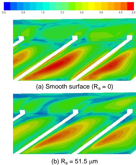
Figure 5 – Skin friction coefficient distribution with the surface roughness variation
