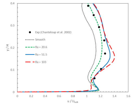
(a) u-velocity
