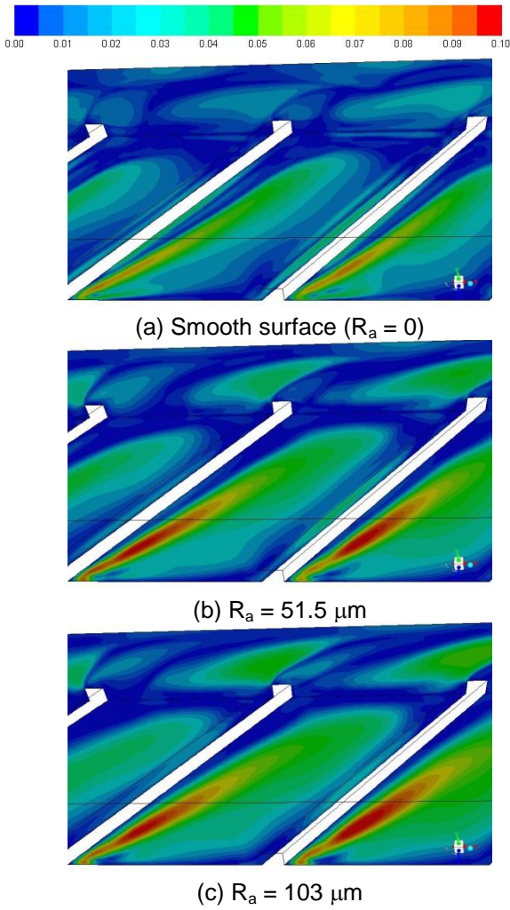
Figure 5 – Skin friction coefficient distribution with the surface roughness variation
