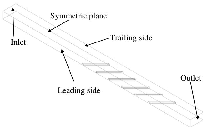
Figure 3 – Computational domain of a Ribbed Duct
