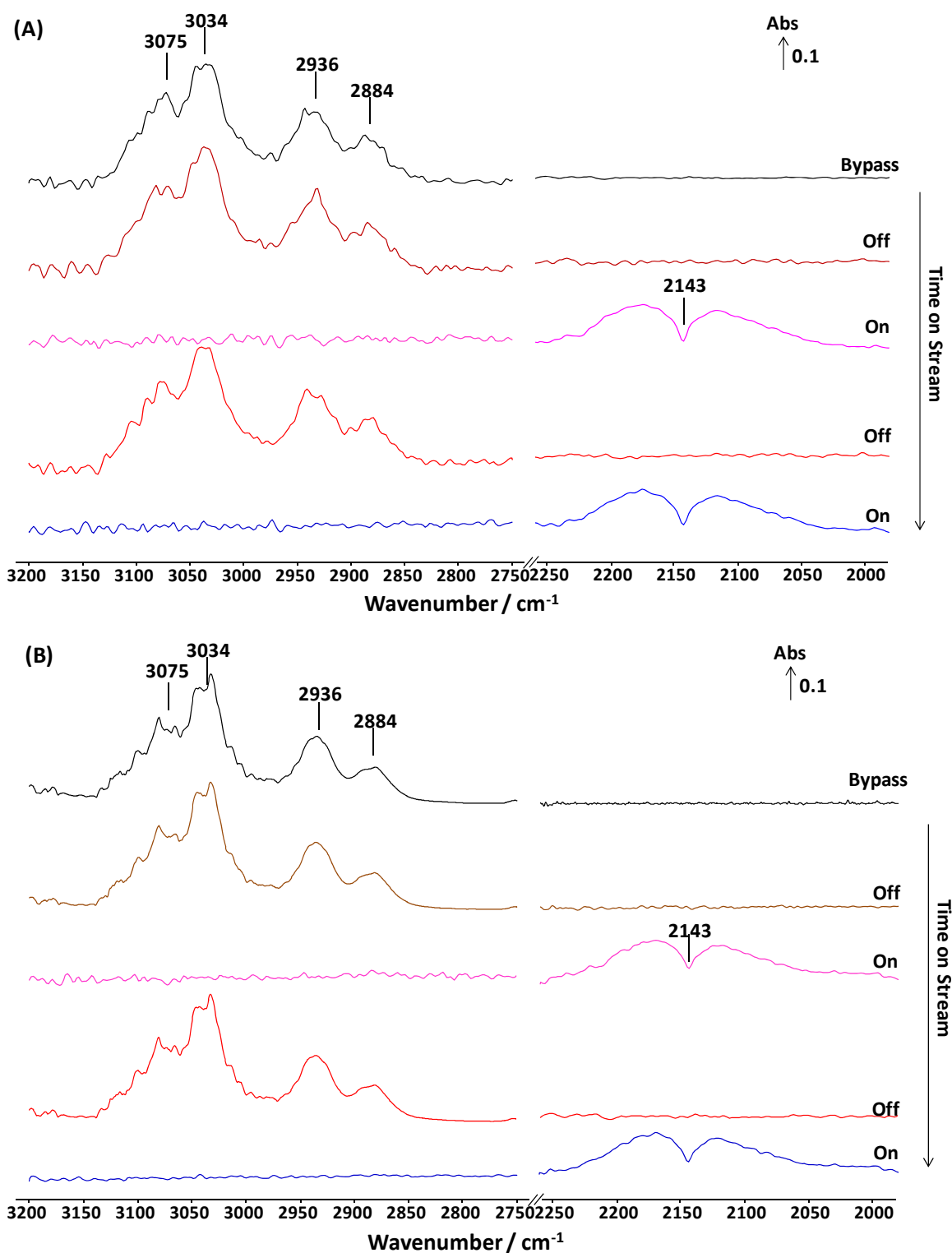
Figure 3. FTIR spectra of gas phase species recorded during switching 7 kV, 19 kHz plasma on and off under toluene-SCR of NO x reaction conditions over 2% Ag/Al 2 O 3 catalyst at (A) 250°C and (B) 25 °C. Feed conditions: 720 ppm NO, 4.3% O 2 , 4340 ppm (as C 1 ) toluene, 7.2% CO 2 , 7.2% H 2 O, He Balance. The total flow rate and space velocity was 276 cm 3 min -1 and 165,600 cm 3 g -1 h -1 , respectively.
