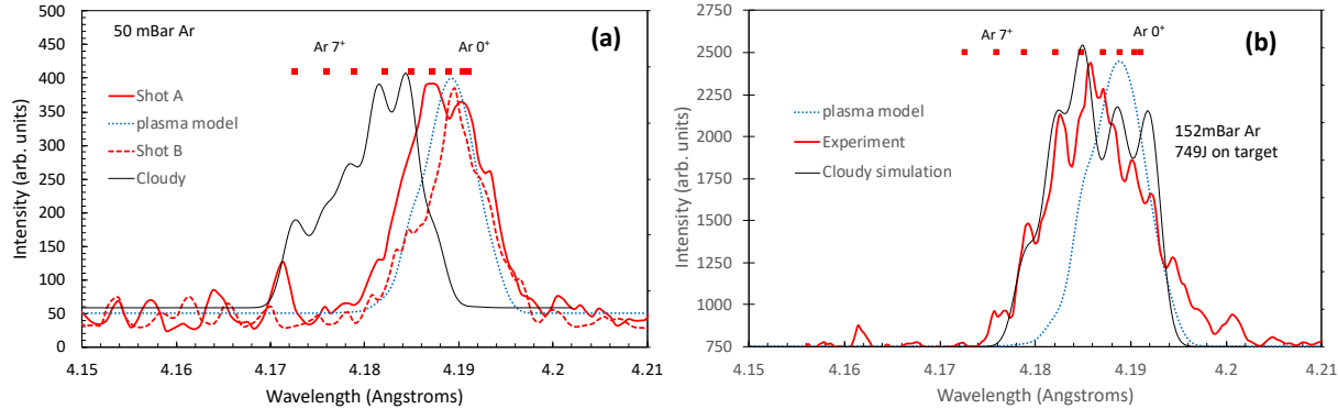
FIG. 5. (a) Lineout from two shots with a 50 mbar gas fill close to the source at z = 0.5-0.7 mm with incident flux \sim 10^{19} \text{ erg cm}^{-2} \text{ s}^{-1} . The images are despeckled before the lineouts are taken (pixels replaced with median of a surrounding 3 \times 3 grid, conserving overall signal). For this lowest pressure case shot-to-shot variation in the profile can be seen more strongly than at higher pressures due to lower signal levels. (b) Raw data lineout (0.5-0.7mm) from a shot with 152 mbar gas fill and a similar incident flux to (a). See the text for discussion of the simulations. In both figures we mark the positions of the expected K- \alpha_1 lines from different ion stages.
