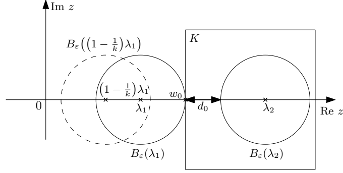
FIGURE 1. The choice of K .
