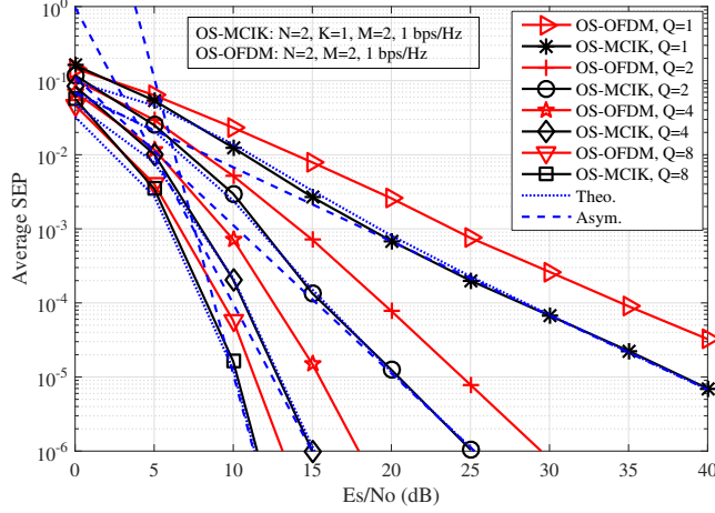
Fig. 2. SEP comparison between OS-MCIK-OFDM with (N, K, M) = (2, 1, 2) and OS-OFDM with (N, M) = (2, 2) , when Q \in \{1, 2, 4, 8\} , at the same data rate of 1 bps/Hz..
