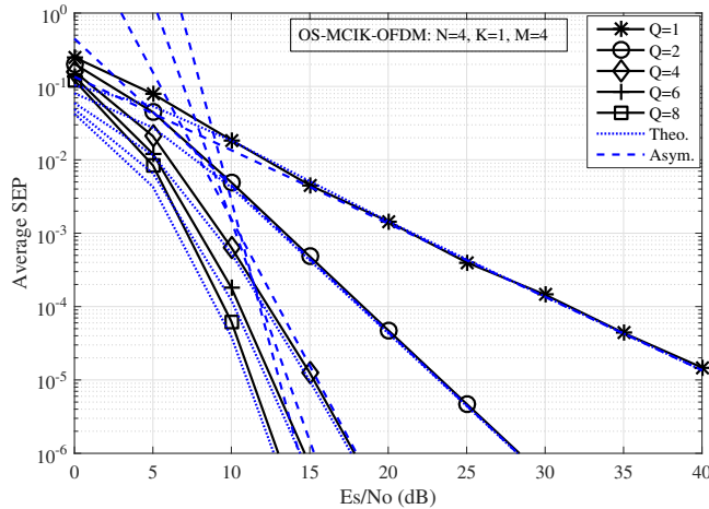
Fig. 1. SEP performance of OS-MCIK-OFDM when (N, K, M) = (4, 1, 4) and Q \in \{1, 2, 4, 6, 8\} .
