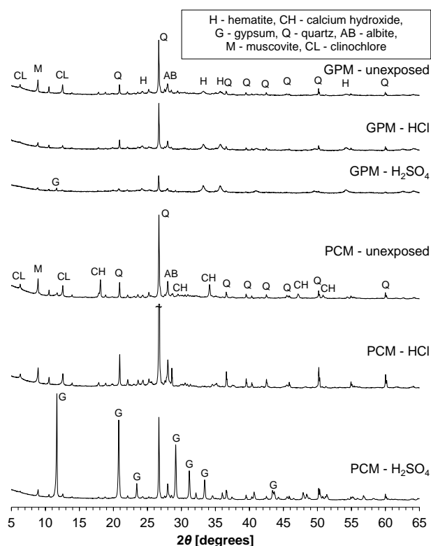
Fig. 8. XRD patterns of unexposed GPM and PCM samples and samples exposed for 8 weeks to HCl and H_2SO_4 solutions.
