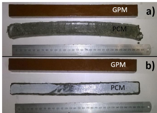
Fig. 2. Visual appearance of GPM and PCM samples after 52 weeks of exposure to 0.352 mol/L solutions of a) \text{Na}_2\text{SO}_4 and b) \text{MgSO}_4 .
