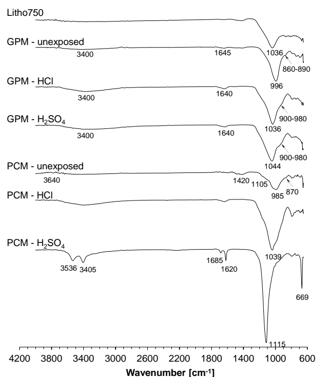
Fig. 9. FTIR spectra of unexposed GPM and PCM samples and samples exposed for 8 weeks to HCl and H_2SO_4 solutions.
