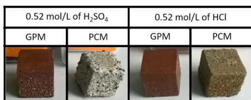
Fig. 6. Visual appearance of GPM and PCM after 8 weeks of exposure to \text{H}_2\text{SO}_4 and HCl acid solutions.
