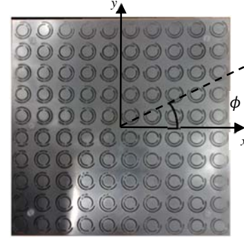
Fig. 2 Reflectarray with azimuthally rotated elements
