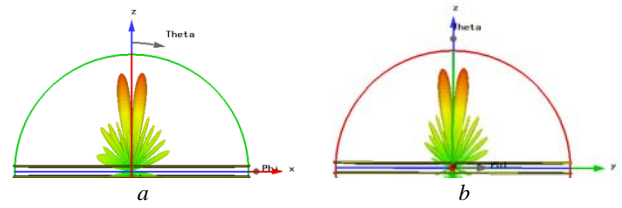
Fig. 3 Simulated reflected far-field pattern of the 10x10 reflectarray excited with plane wave polarized along the x-axis at 10.4GHz
