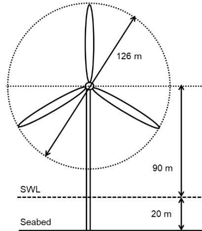
Figure 1. Main dimensions of the NREL 5 MW Wind Turbine.
