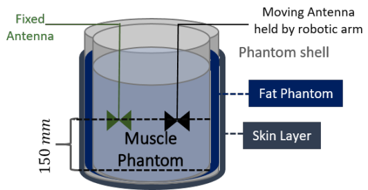
Fig. 3. Illustration of experimental setup showing tissue layers.
