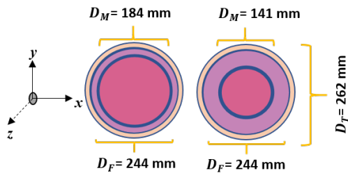
Fig. 1. Schematics of Phantom 1 (left) and Phantom 2 (right).
