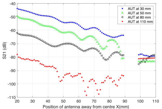
Fig. 4. Measured forward path gain |S_{21}| in Phantom 1 .
