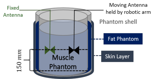
Fig. 3. Illustration of experimental setup showing tissue layers.
