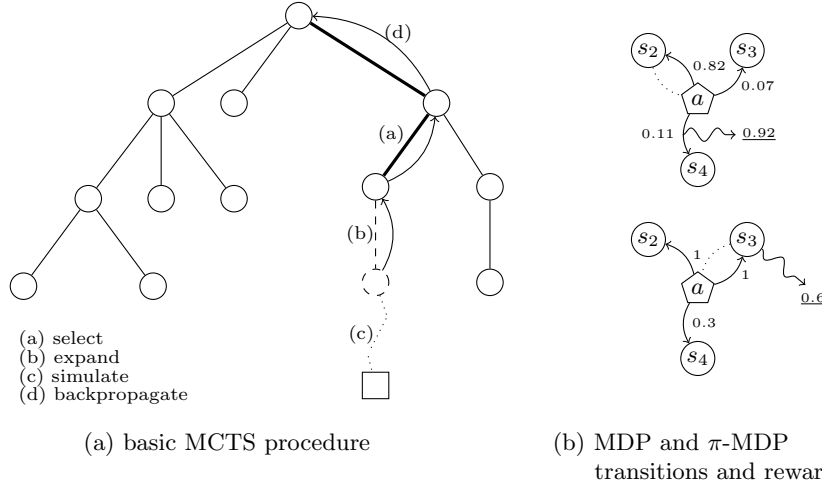
Fig. 1: (left) basic MCTS procedure with the 4 distinct phases in each iteration (right) MDP and \pi -MDP differences, where transitions are either probabilities or possibilities, rewards are over transitions, and preferences are over states
