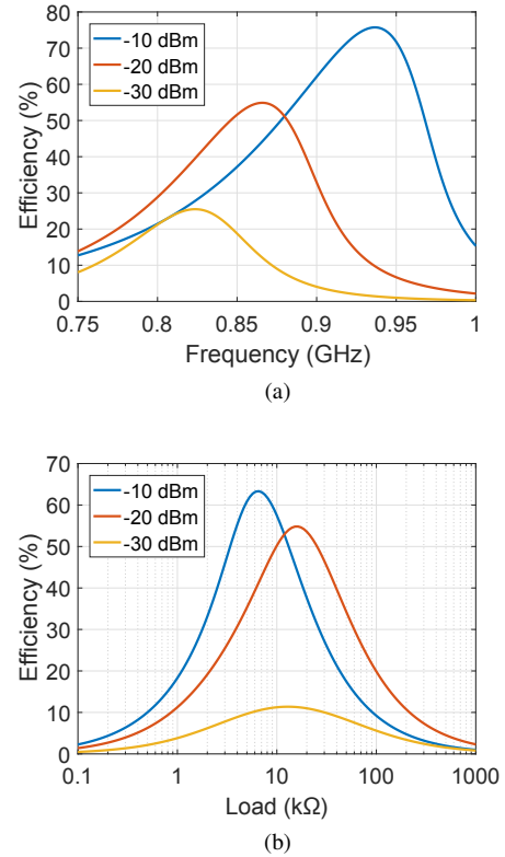
Fig. 3. Simulated rectifier’s efficiency versus frequency (a) and load (b) for various levels of power input: when the frequency varies the load is fixed at 15.4 \text{ k}\Omega , while when the latter varies, the frequency is fixed at 868 MHz. At both cases, Z_a = 54.6 + j707.6 \Omega .
