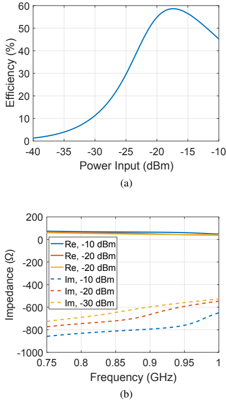
Fig. 2. Simulated rectifier’s RF-to-dc efficiency versus power input at 868 MHz (a) and the real (Re) and the imaginary (Im) part of the rectifier’s input impedance versus frequency for various levels of power input (b). The load R at both cases is 15.4 \text{ k}\Omega and for the source is Z_a = 54.6 + j707.6 \Omega .
