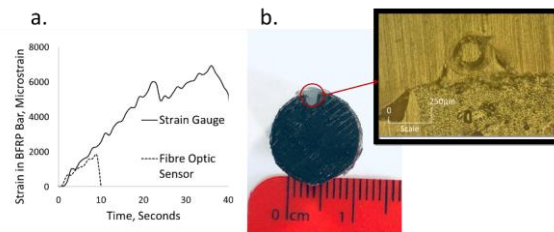
Fig. 3 Test Results for Specimen 12-C1-A-S3. (a) Comparison of Strains between FOS and ERSG (b) Microscope Image of the Specimen.
