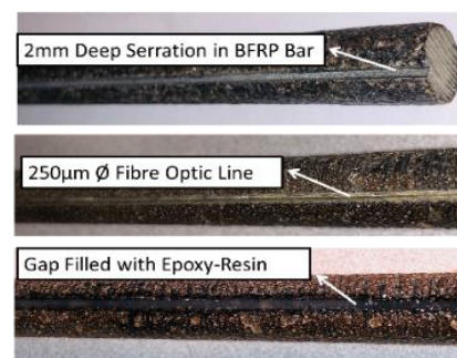
Fig. 1 Preparation of Specimen 12-C1-A-S3
