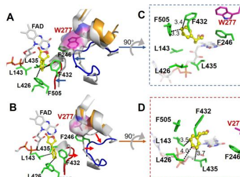
Fig. 2 Comparison of MD structures of WT CHMO and its mutants. (A) F277W complexed with ( R )- 2a ; (B) F277V complexed with ( S )- 2a ; (C), (D) A rotation about 90 degrees into the page from the perspective of (A), (B). WT is shown with pale gray cartoon as a reference; Ligand 2a is shown with ball and sticks (yellow carbon atoms); The crucial position 277 is shown with sticks and surface. The unit of distances is in Å.
