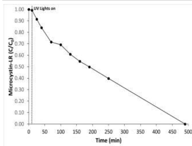
Figure 11: The kinetic profile of photocatalytic degradation microcystin-LR (1mg in 200 \text{cm}^3 of artificial fresh water) performed with pod 4 containing \text{TiO}_2 coated glass beads. The loading of \text{TiO}_2 is 250 mg per 1g of coated glass beads. The LED array was operated at V_f = 12 dcV and I_f = 0.09 A (1.1 W). The delay time for dark absorption was 10 min.
