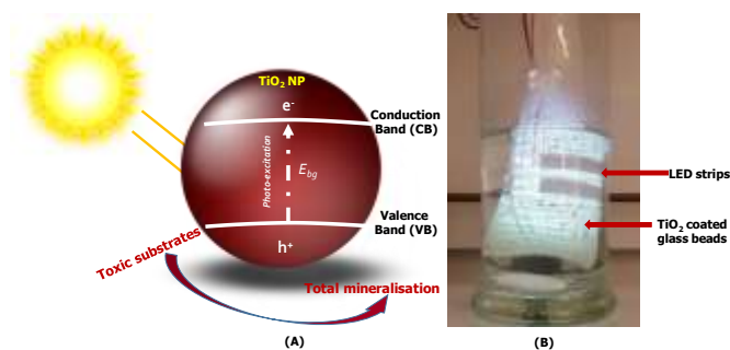
Figure 1: (A): Illustration of the 'hole forming' photochemical process of TiO 2 that is responsible for photo-catalytic destruction of toxic substrates such as microcystins; (B) our design of a pod with a LED attachment containing glass beads coated with TiO 2 -NPs
