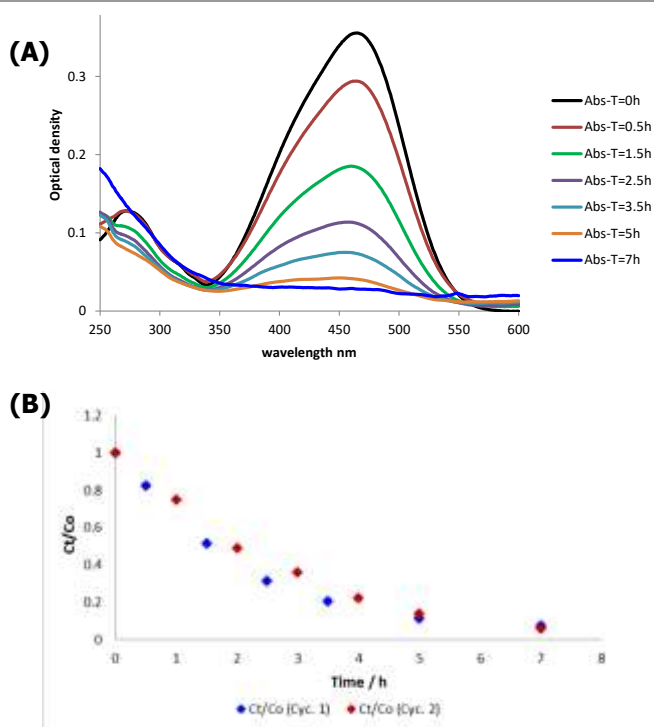
Figure 4: (A), Degradation of the methyl orange dye is seen, with time, by the demise of the absorption band centred at 465 nm; (B), red and blue curves show the kinetic profile for two repeated cycles using the TiO 2 supported glass wool. Ct and Co refer to OD (465 nm) at time=t and time=0, respectively
