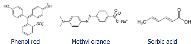
Scheme 1: Compounds used for the photocatalytic degradation study
