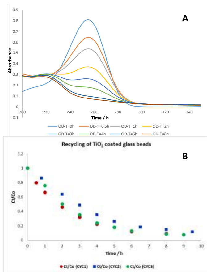
Figure 10: (A), a set of UV-spectra obtained for the 1st run of sorbic acid degradation utilising pod 6 with glass beads. Initial [Sorbic acid] = 3.488 \times 10^{-5} M; (B), kinetic profiles of 3 photocatalytic degradation runs carried out with pod 4 with the same coated glass beads. Ct and Co refer to OD (256 nm) at time=t and time=0, respectively
