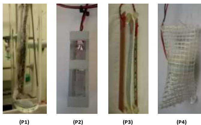
Figure 3: P1 the inner perforated tube contains two LED strips with TiO 2 coated glass wool placed in between; P2 rectangular shape pod, made of Perspex, with LED strips attached to inner walls where any TiO 2 supported materials can be housed; P3 TiO 2 coated glass fibre tape placed between two UV LED strips; P4 a pod made up of fibre glass mesh where wired UV LED strips are attached inside. TiO 2 coated glass beads or glass wool may be placed inside.
