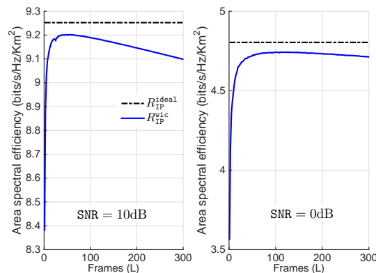
Fig. 3. Area spectral efficiency of MRC receivers as a function of frames L . In this example, N = 20 , the number of frames that IQI remains invariant over is B = 1000 , the propagation channel parameters are \sigma = 10 dB and pathloss \alpha = 3.8 .
