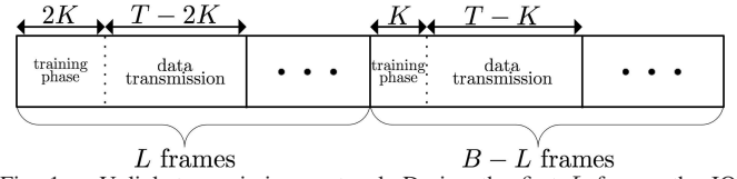
Fig. 1. Uplink transmission protocol: During the first L frames the IQI coefficients: \mathbf{K}_1 , \mathbf{K}_2 and the channel \mathbf{Y} are jointly estimated with pilot length \tau = 2K . After estimating the IQI coefficients, and employing the IQI compensation scheme the channel can be estimated directly from (37) during the next B - L frames with pilot length \tau = K .
