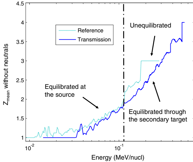
FIG. 2 (color online). Z_{\text{mean}} for carbon ions as measured by the “reference” TP1 and “transmission” TP2 after 100 nm of aluminum target at 300 K. The error is \pm 0.005 MeV/nuc for the energy and the uncertainty is \pm 0.1 for the mean charge.
