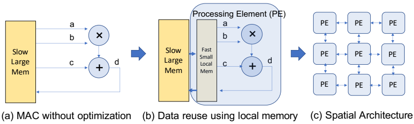
Fig. 9. Multiply-and-accumulate dataflow.
