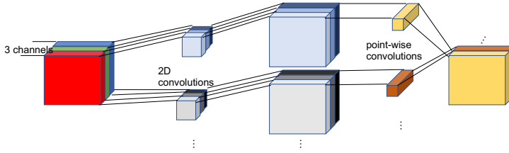
Fig. 5. Depth-wise convolution used in [83].
