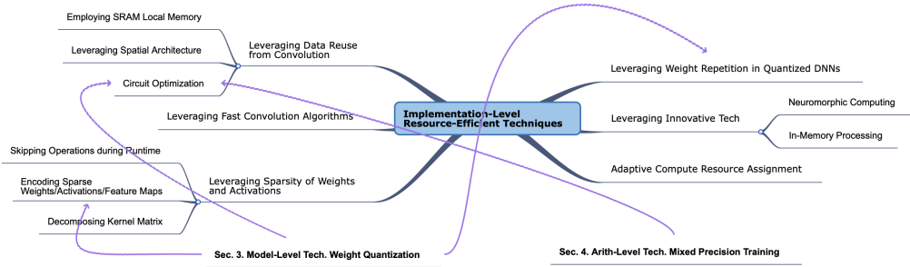
Fig. 8. Categorization of implementation-level resource-efficient techniques.
