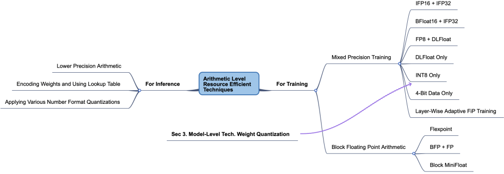
Fig. 7. Categorization of arithmetic-level resource-efficient techniques.
