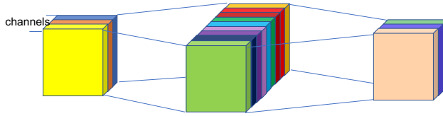
Fig. 6. Bottleneck layer block used in [142].
