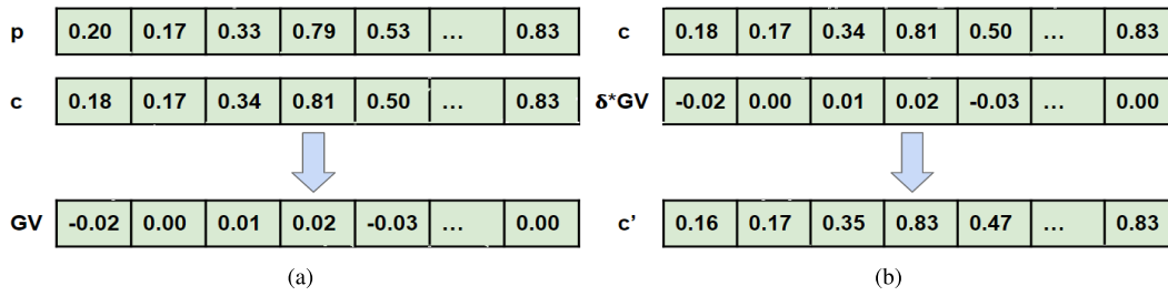
FIGURE 1. Example of genome vector (GV) generated using a parent and a child genome. Here \delta is one.
