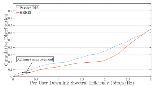
Fig. 3: The cumulative distribution of the SE per user for passive RIS and HR-RIS-aided systems.
