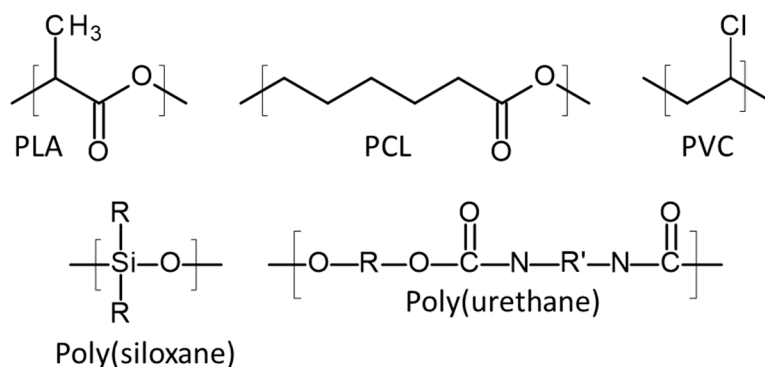
Figure 6. Chemical structures of poly(lactic acid) (PLA), poly(caprolactone) (PCL), poly(vinyl chloride) (PVC), poly(siloxane), and poly(urethane).
