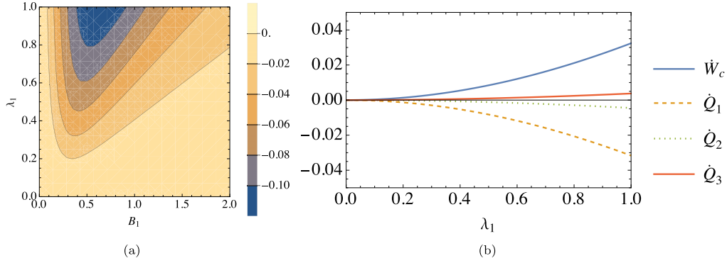
FIG. 7. (a) Contour plot of \dot{Q}_1 in units of T_1 \gamma_1 as a function of B_1 and \lambda_1 when T_1 = T_2 = T_3 = 6 . (b) Plot of all thermodynamic quantities in terms of \lambda_1 for a fixed value of B_1 = 2 , the rest of the parameters are \gamma_1 = 8.7 \times 10^{-3} , \gamma_2 = 5.7 \times 10^{-3} , and \gamma_3 = 7.5 \times 10^{-3} .
