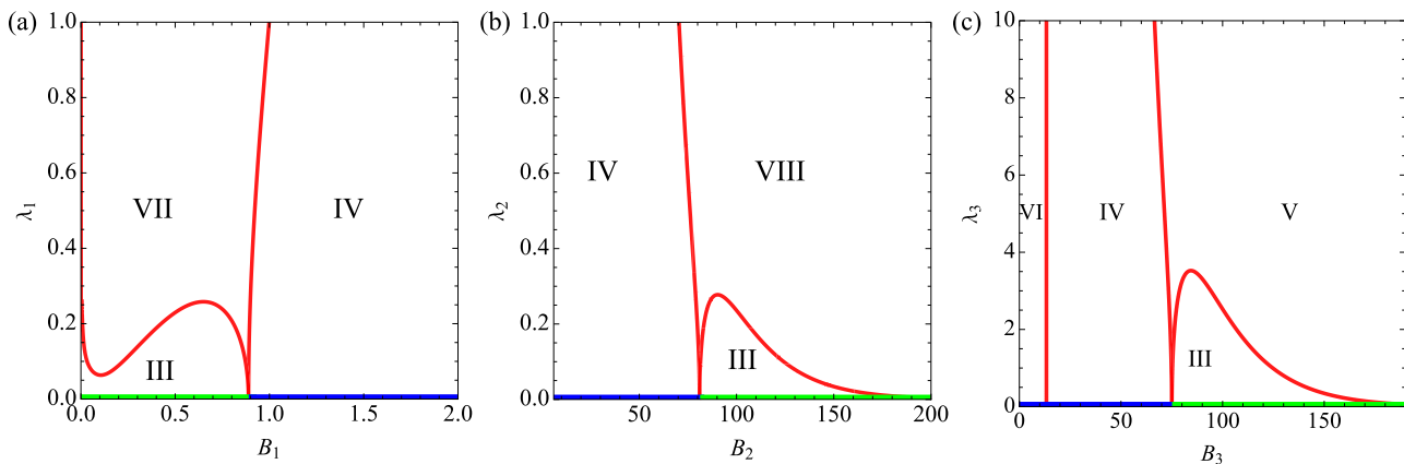
FIG. 2. Operational diagram for the functioning of the machine in the resonance case for: (a) coherence in the cold bath, with B_2 = 12 ; (b) coherence in the intermediate bath with B_1 = 6 ; and (c) coherence in the hot bath with B_1 = 6 . The green and blue horizontal lines, for \lambda_i = 0 , correspond to the regimes I and II, respectively. The red lines serve as boundaries that mark the shifts between the regimes, which are made possible by the input coherence in the environmental units. The rest of the parameters are T_1 = 1.0 , T_2 = 6.0 , T_3 = 10.0 , \gamma_1 = 8.7 \times 10^{-3} , \gamma_2 = 5.7 \times 10^{-3} , and \gamma_3 = 7.5 \times 10^{-3} .
