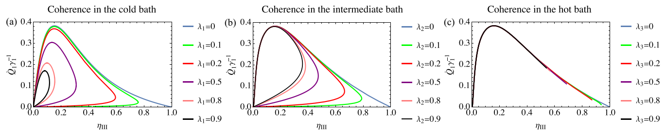
FIG. 3. Quantifying the performance of the machine in regime III via its efficiency \eta_{\text{III}} in terms of the cooling power \dot{Q}_1 in units of T_1\gamma_1 for when coherence is in (a) the cold bath, with B_2 = 9.5 ; (b) the intermediate temperature bath B_1 = 1.24 ; and (c) the hot bath with B_1 = 1.24 . The rest of the parameters are T_1 = 1.0 , T_2 = 2.0 , T_3 = 60.0 , \gamma_1 = 8.7 \times 10^{-3} , \gamma_2 = 5.7 \times 10^{-3} , and \gamma_3 = 7.5 \times 10^{-3} .
