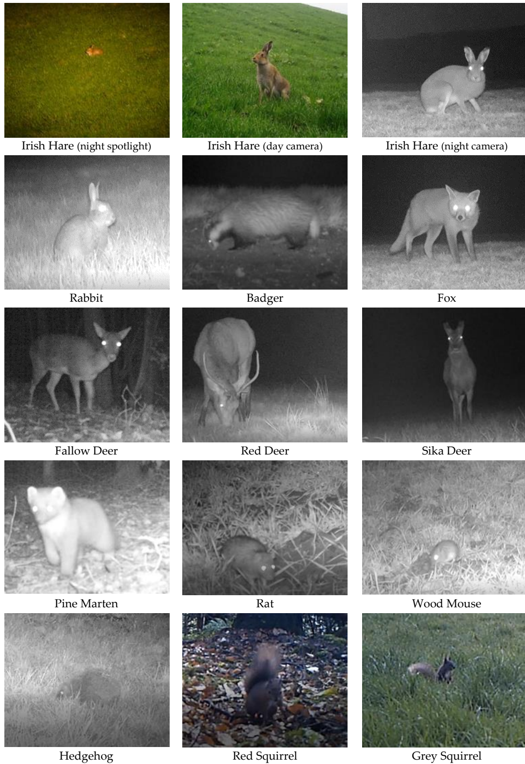
Figure 13 Images of species detected during camera trap surveys including an example of an Irish Hare during the pilot spotlight survey and on camera traps during both day (colour) and night (black and white).
