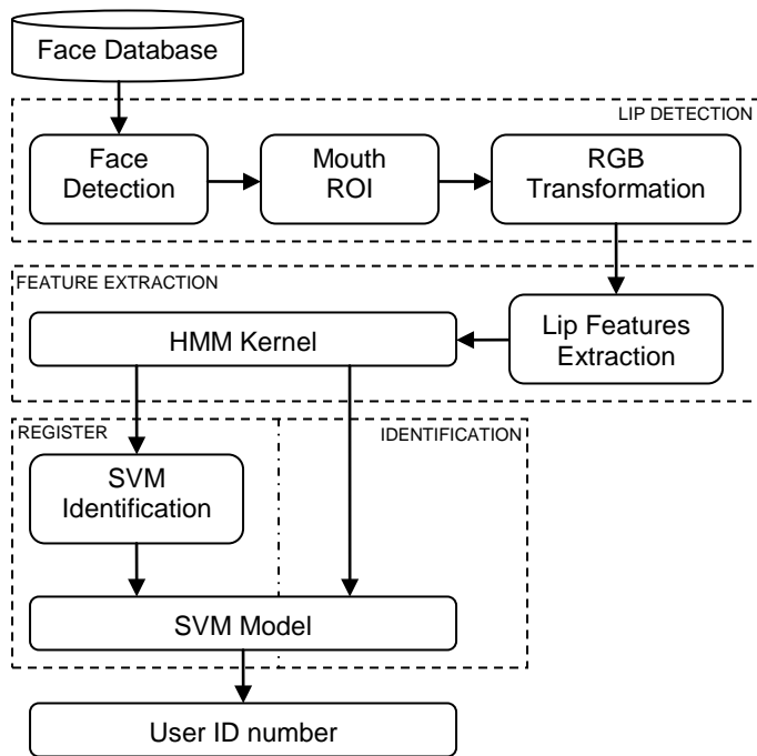
Fig. 1. Block Diagram of the proposed approach.
