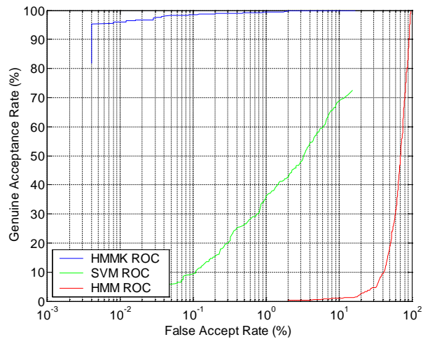
Fig. 7. ROC curves for the RaFD dataset using 2 training samples per class (better viewed in color).
