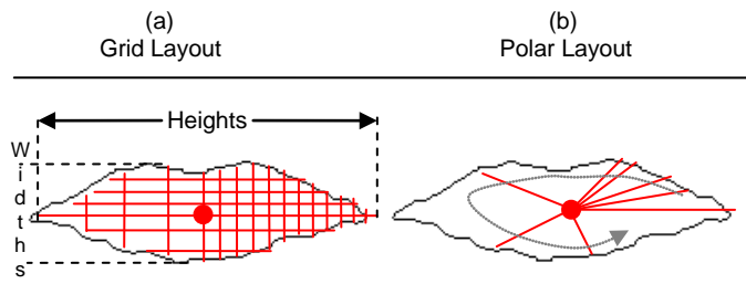
Fig. 4. Geometrical-sequential Features: Rectangular grid (a) and Polar grid (b).
